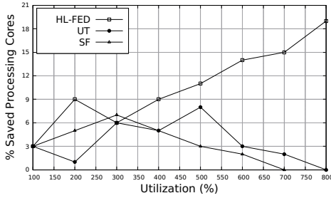
Fig. 6. Simulation results showing the percentage of saved processing cores as a function of utilization for DAGs with high density values and high heavy DAG count in the task set.
